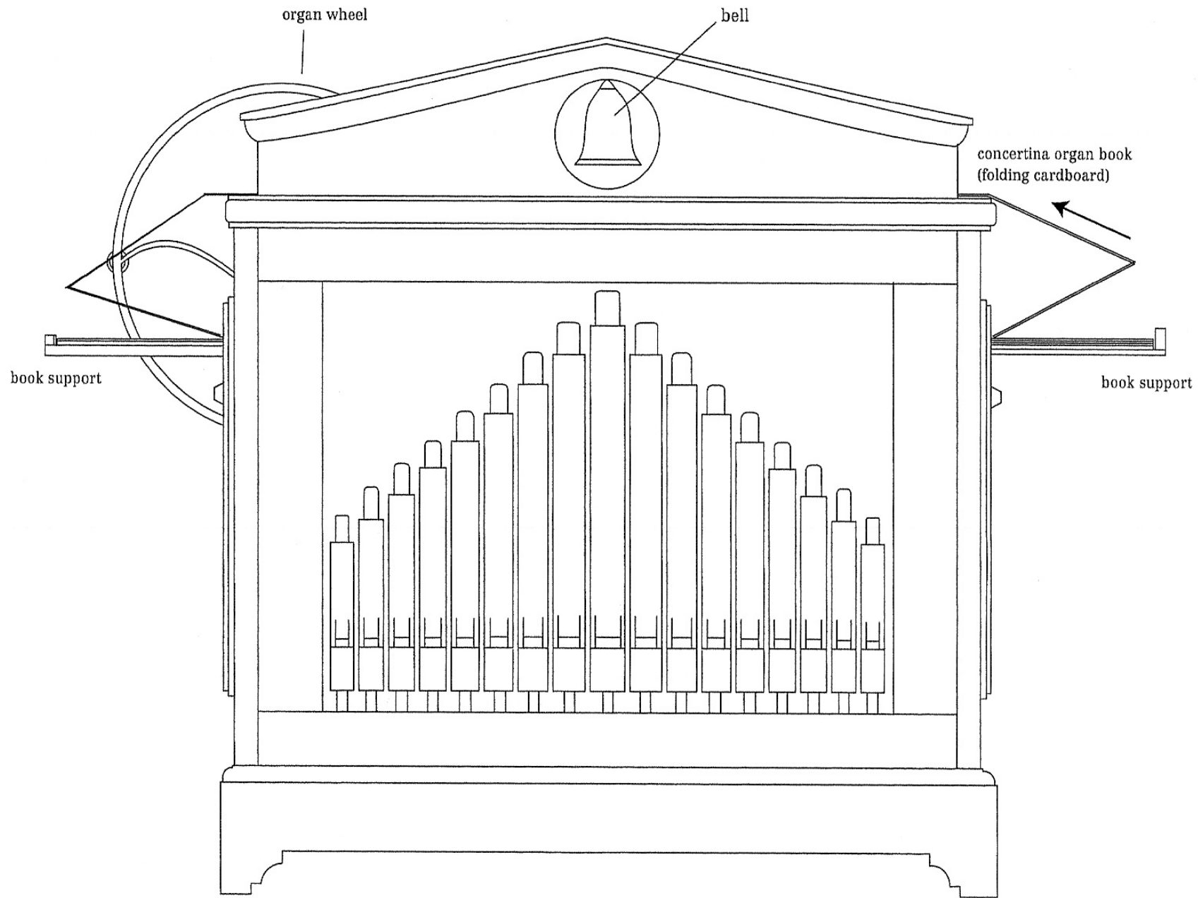
Drawing 1, Front view of small barrel organ
