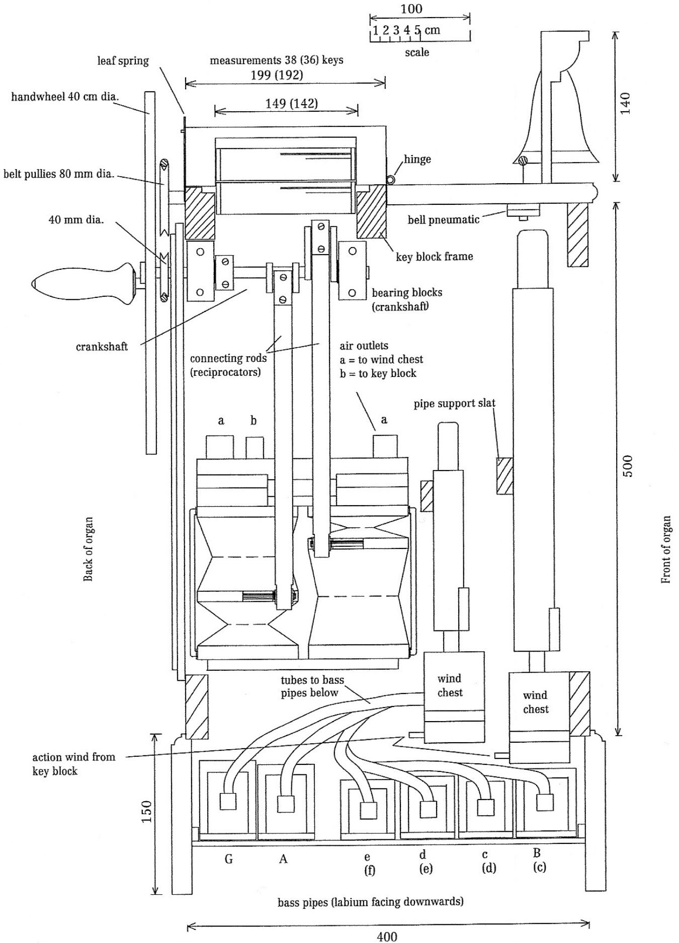
Drawing 3, Sectional side view of barrel organ
